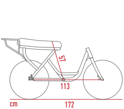
E-bike dimensions
