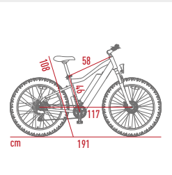
E-bike dimensions
