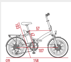
E-bike dimensions
