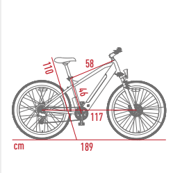
E-bike dimensions
