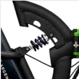
Full Suspension
