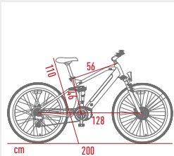
E-bike dimensions
