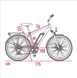
E-bike dimensions
