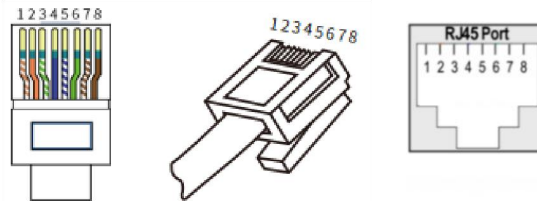
Inverter CAN
