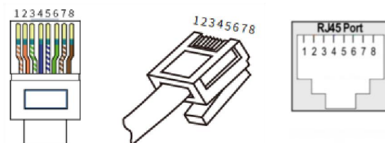
Battery CAN
